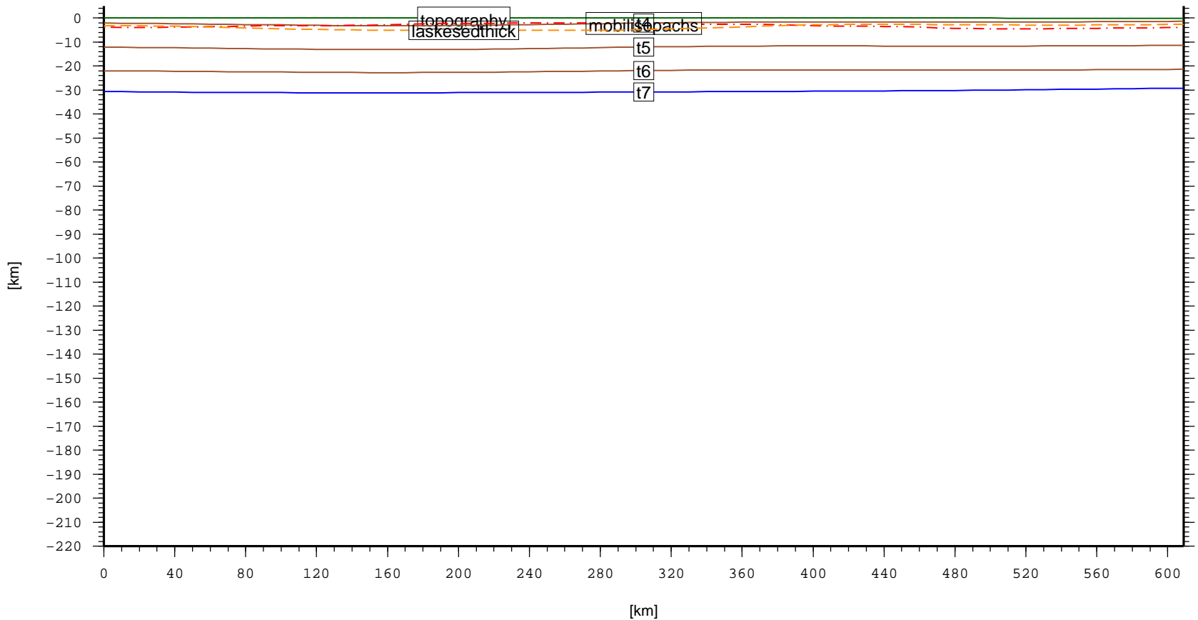
Cross section – SUN.MalayBasin (topo, laske sedthick, t4, t5, t6, t7)
