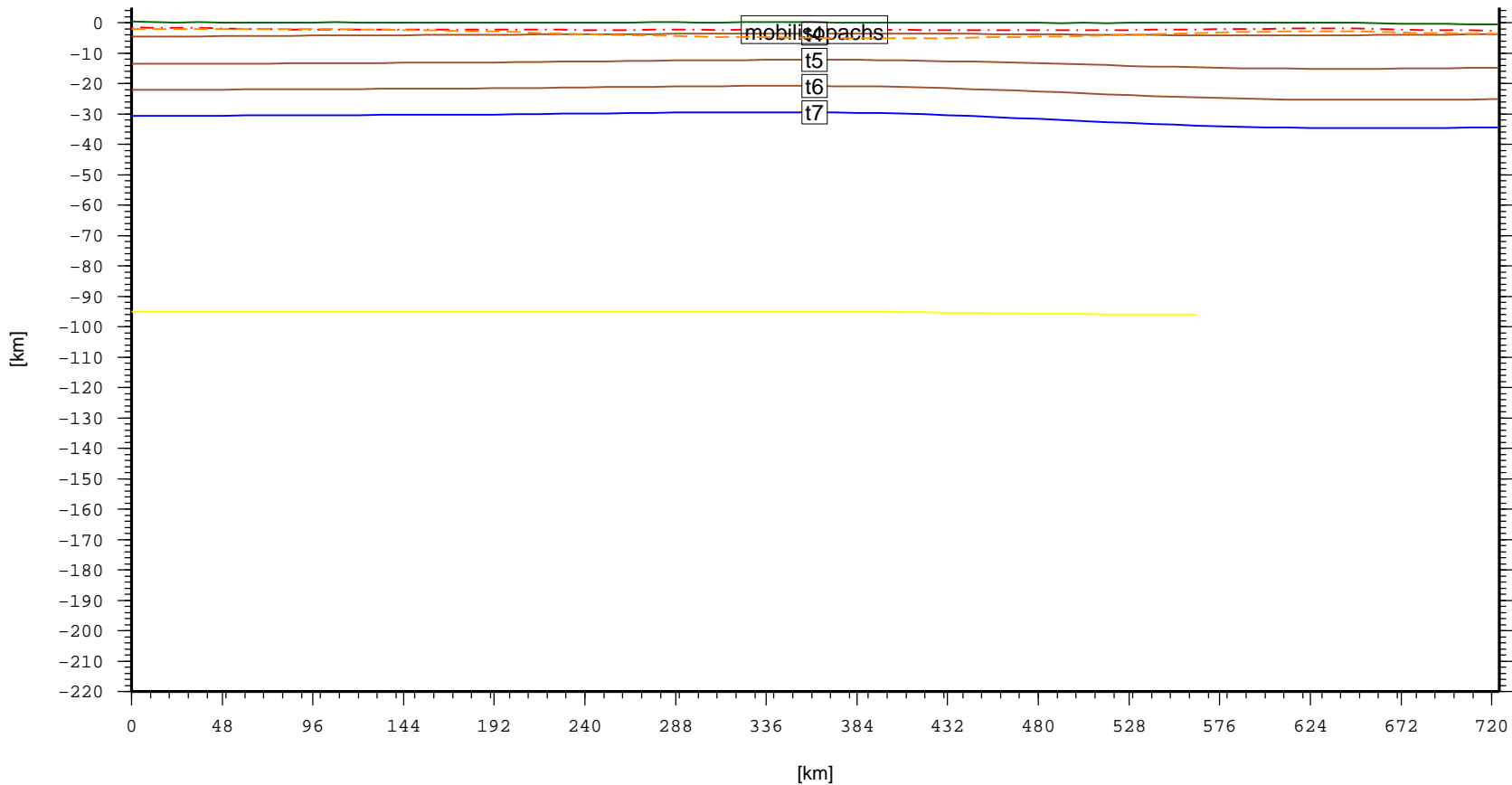
Cross section – SUN.EastJavaBasin (topo, laske sedthick, t4, t5, t6, t7)
