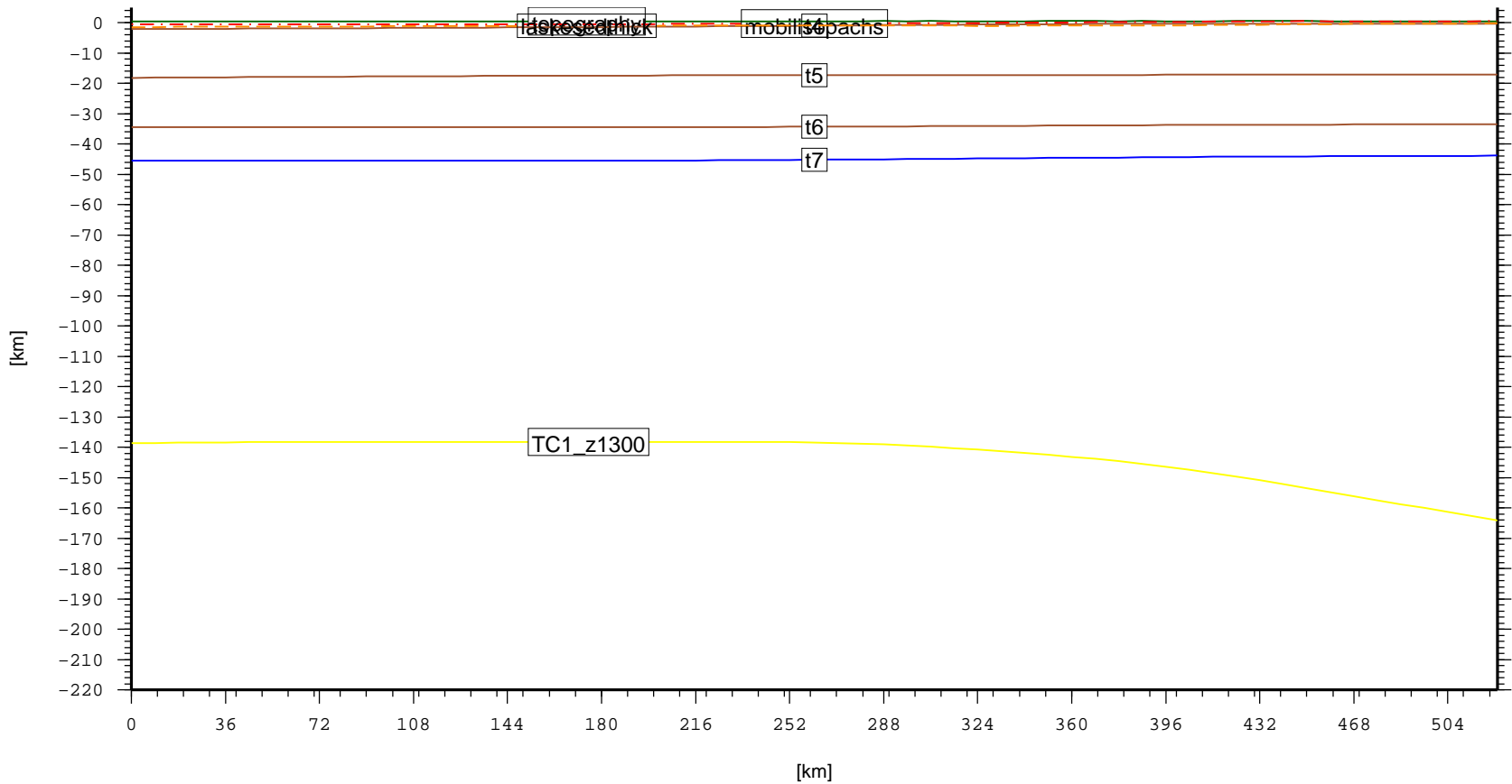
Cross section – NAM.SalinaBasin (topo, laske sedthick, t4, t5, t6, t7)
