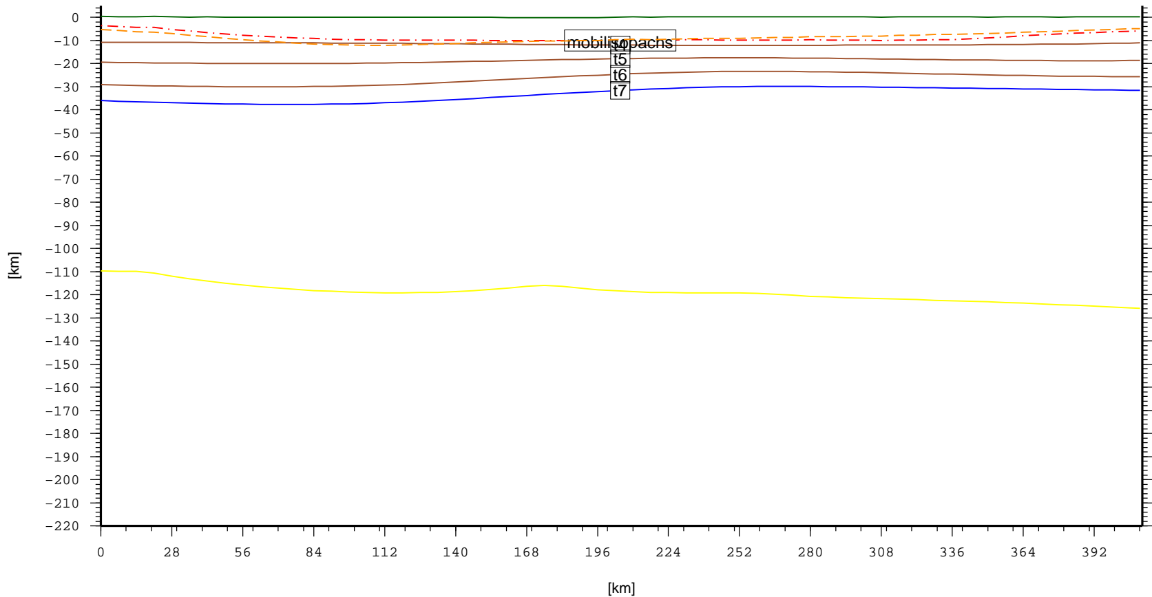
Cross section – CAS.Indol–KubanBasin (topo, laske sedthick, t4, t5, t6, t7)
