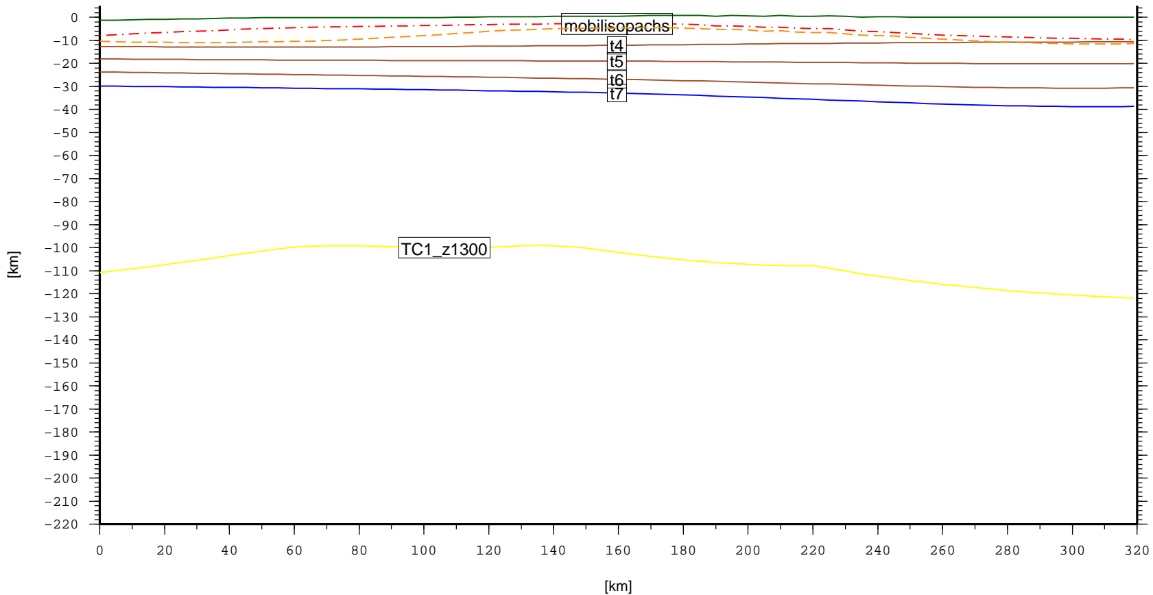
Cross section – CAS.CrimeaFoldBelt (topo, laske sedthick, t4, t5, t6, t7)
