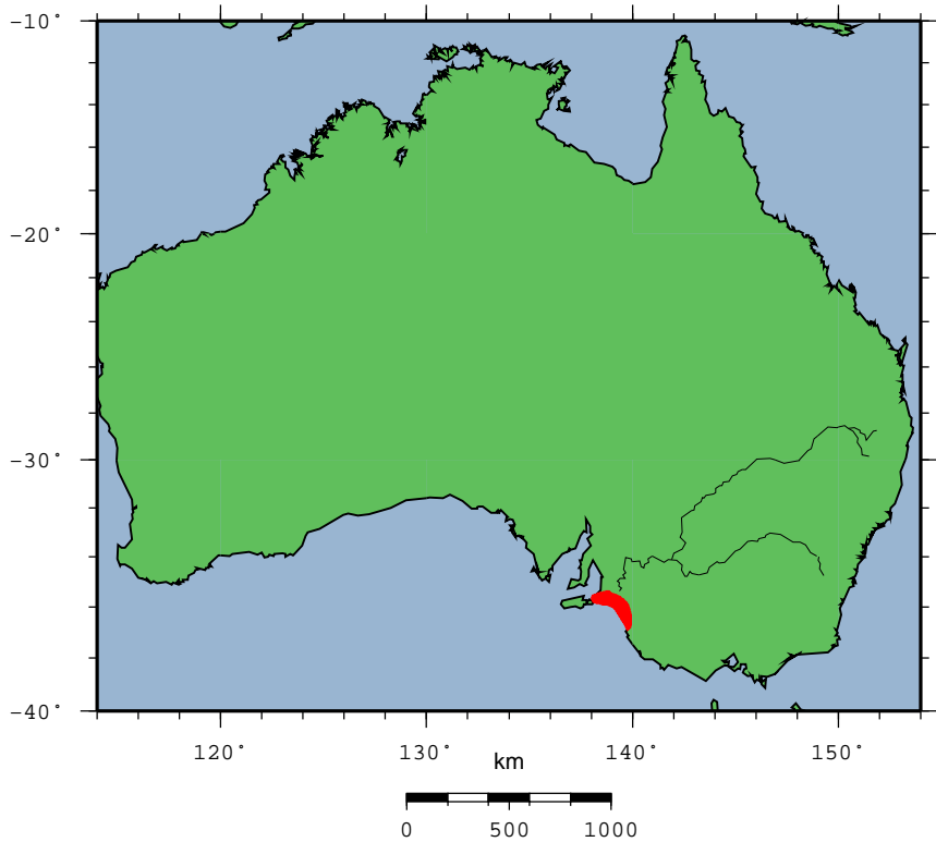
Location map AUS.TroubridgeBasin.
