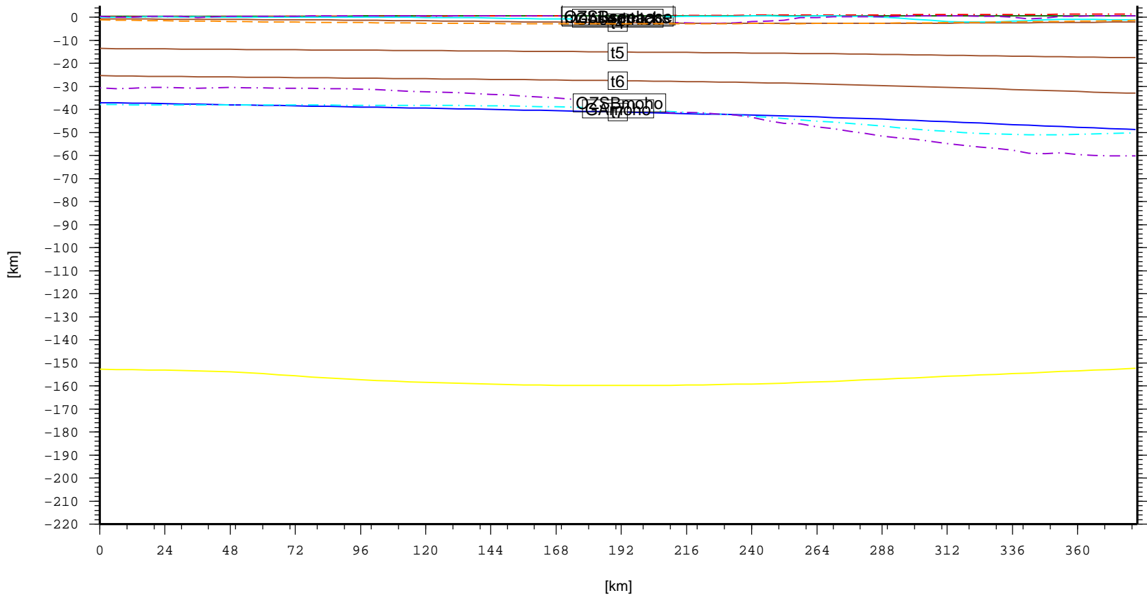
Cross section – AUS.NgaliaBasin (topo, laske sedthick, t4, t5, t6, t7)
