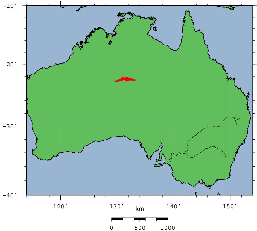
Location map AUS.NgaliaBasin.
