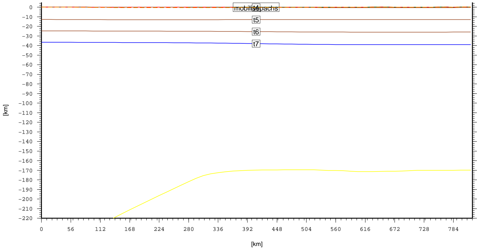
Cross section – ARC.FoxeBasin (topo, laske sedthick, t4, t5, t6, t7)
