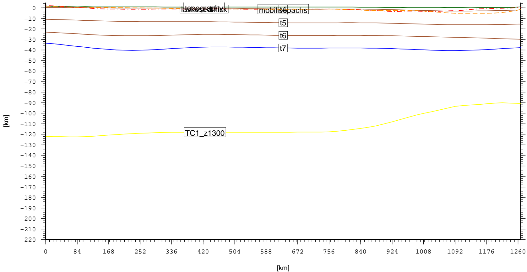
Cross section – ARA.WesternArabianProvince_ArabianBasin (topo, laske sedthick, t4, t5, t6, t7)
