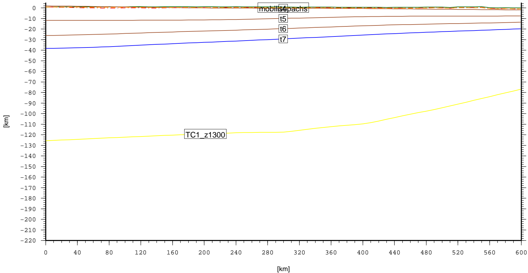
Cross section – ARA.Sir–SayunBasin (topo, laske sedthick, t4, t5, t6, t7)
