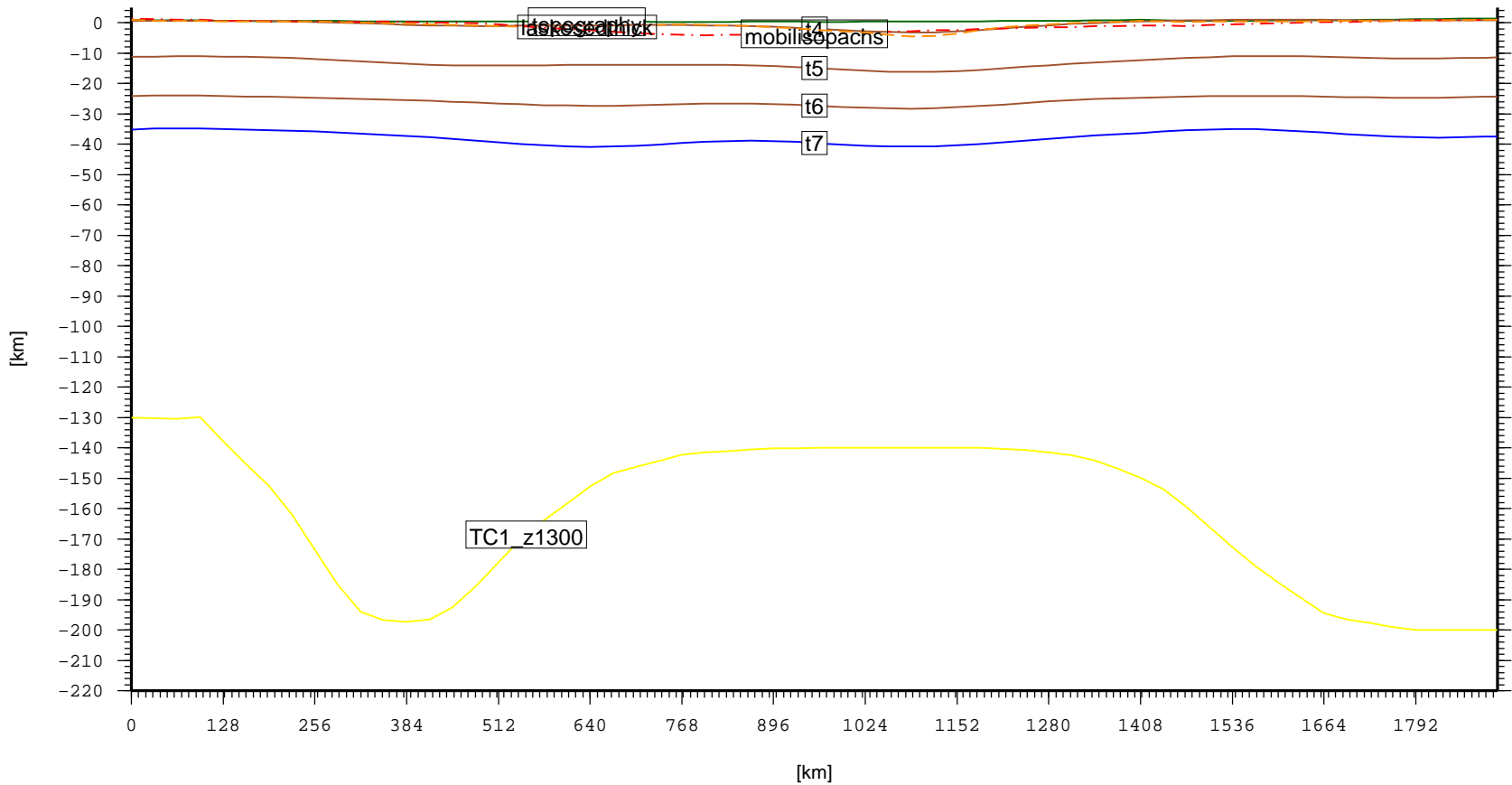
Cross section – AFR.ZaireBasin (topo, laske sedthick, t4, t5, t6, t7)
