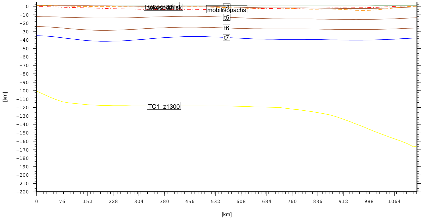
Cross section – AFR.MugladBasin (topo, laske sedthick, t4, t5, t6, t7)
